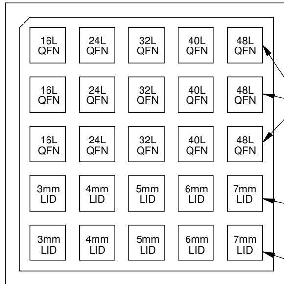
2-INCH WAFFLE PACK TOP VIEW
