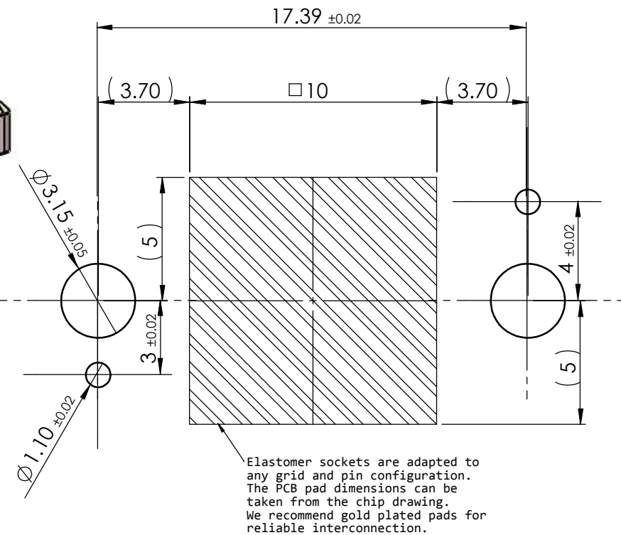
PCB LAYOUT
