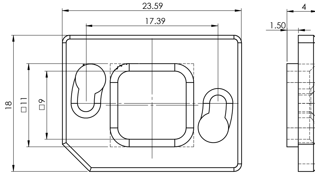
RETENTION FRAME
