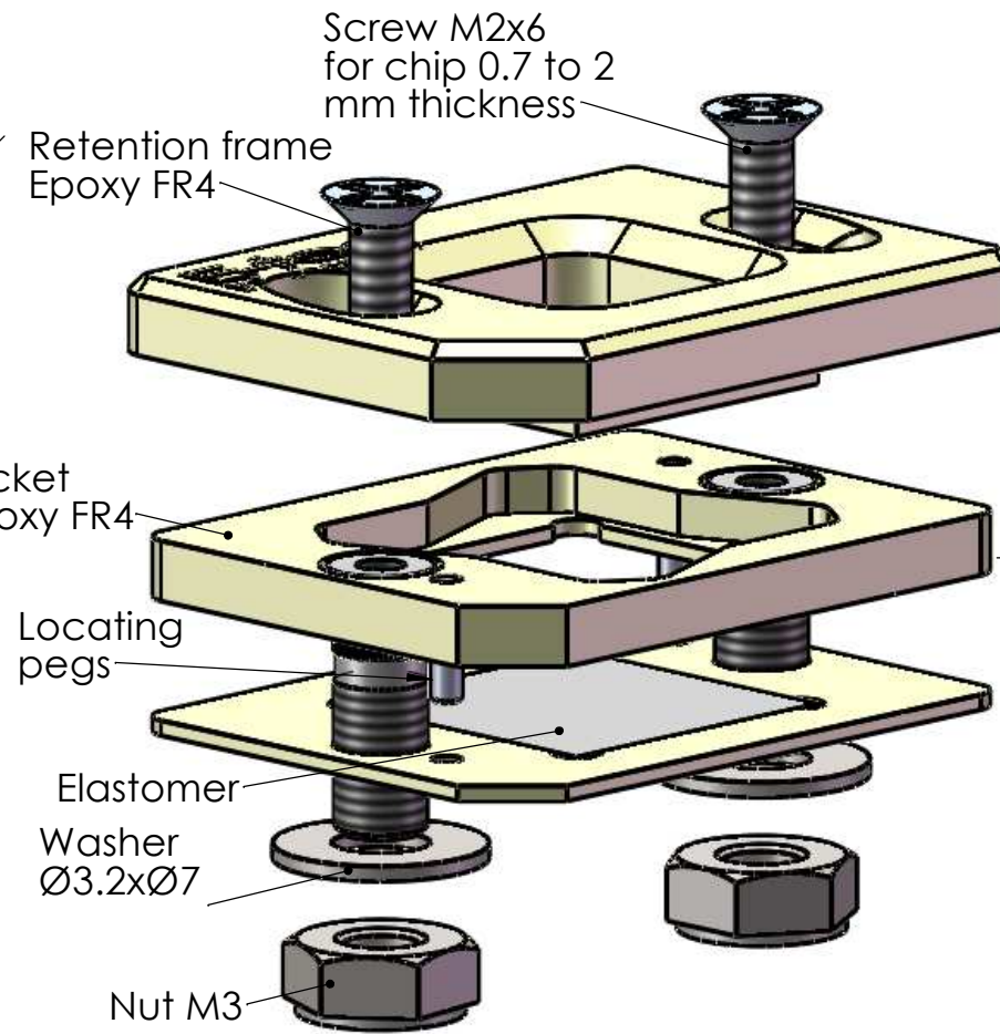
RETENTION FRAME
