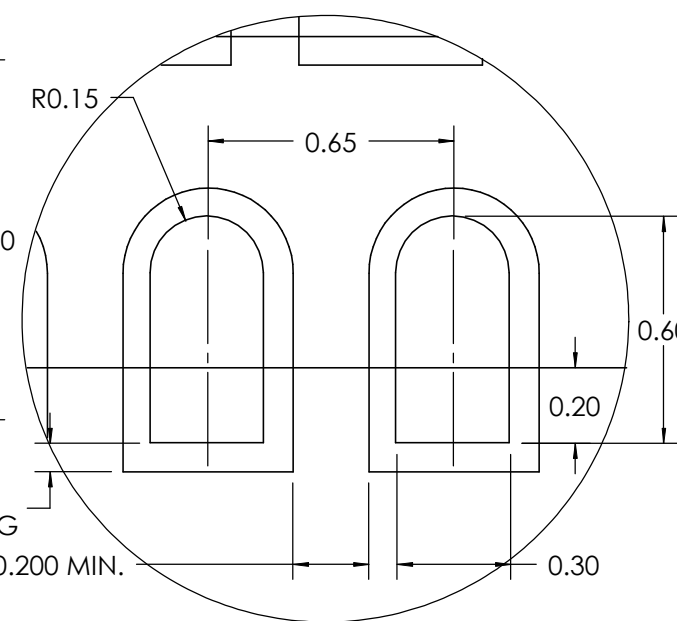
DETAIL A SCALE 50 : 1
