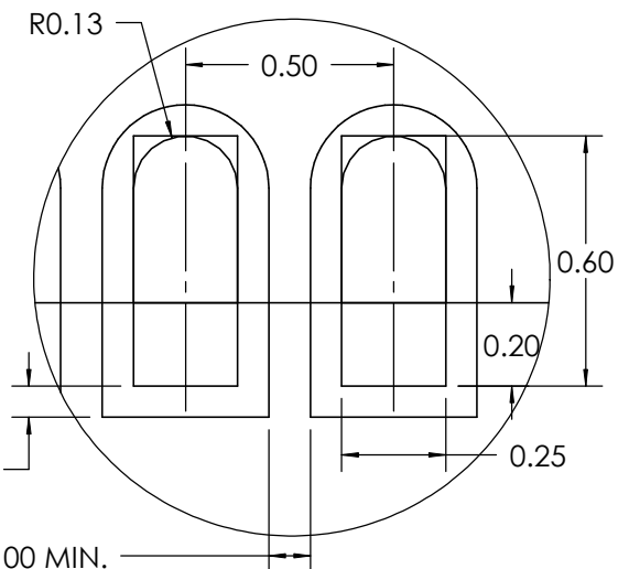
DETAIL A SCALE 50 : 1
