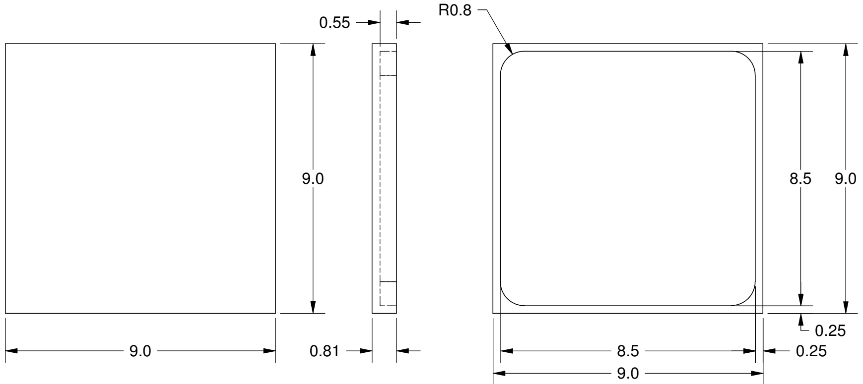
TOP VIEW CLOSED SIDE
